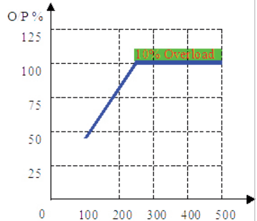
*Load Curve
